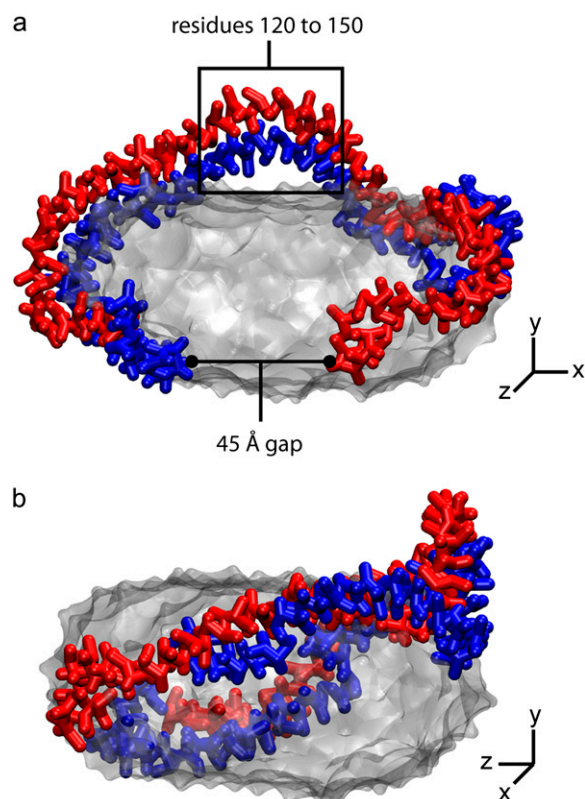
FIGURE 3 Solar-flares discoidal HDL model after 750 ns of coarse-grained molecular dynamics simulation. Two views of the HDL particle are shown, one looking directly at the protein N- and C-termini (a), and the other rotated by 90° (b). The two apolipoprotein strands are shown in red and blue. The POPC lipids and cholesterol molecules are shown as a solid transparent gray surface. Due to the unfavorable orientation of the apolipoprotein strands to the lipid bilayer, a gap (a) has opened up between the N- and C-terminus of the proteins and the lipids in this area form a micellelike structure. A gap has also opened up between the apolipoprotein strands and the lipid bilayer in the region between residues 120 and 150, allowing water to infiltrate and the lipids are also micellelike (a). Additionally, in numerous locations one of the protein strands has rotated so that it no longer makes contact with the lipid bilayer but rather interacts only with the other protein strand (b).
