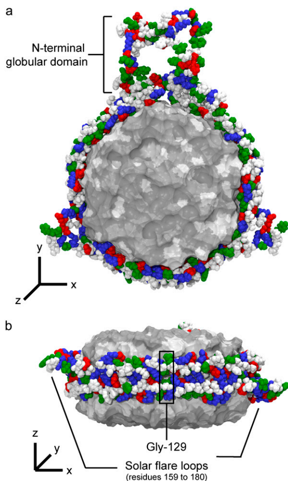
FIGURE 1 A solar-flares discoidal HDL model with proteins colored by residue type. A top-view (a) and side-view (b) of a solar-flares HDL model (3). Protein residues are colored by residue type as follows: hydrophobic residues in white, polar residues in green, basic residues in blue, and acidic residues in red. The lipid bilayer containing 200 POPC lipids and 20 cholesterol molecules is shown as a solid surface colored in gray. Solar flares orient the hydrophobic face of the amphipathic apolipoprotein A-I proteins facing out toward the aqueous environment.
